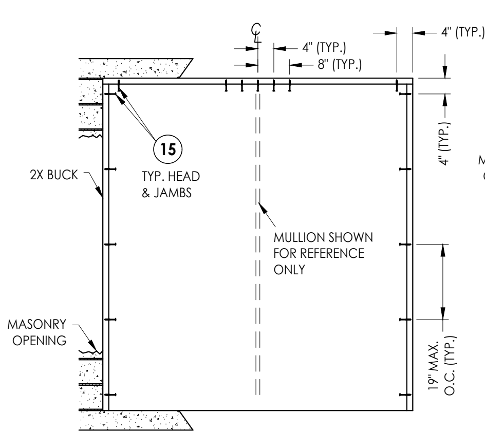
BUCK ANCHORING
