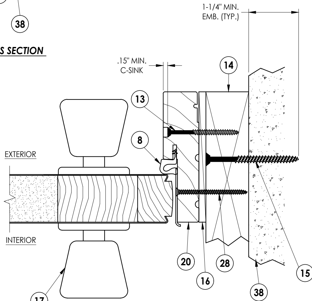
3 3 HORIZONTAL CROSS SECTION
